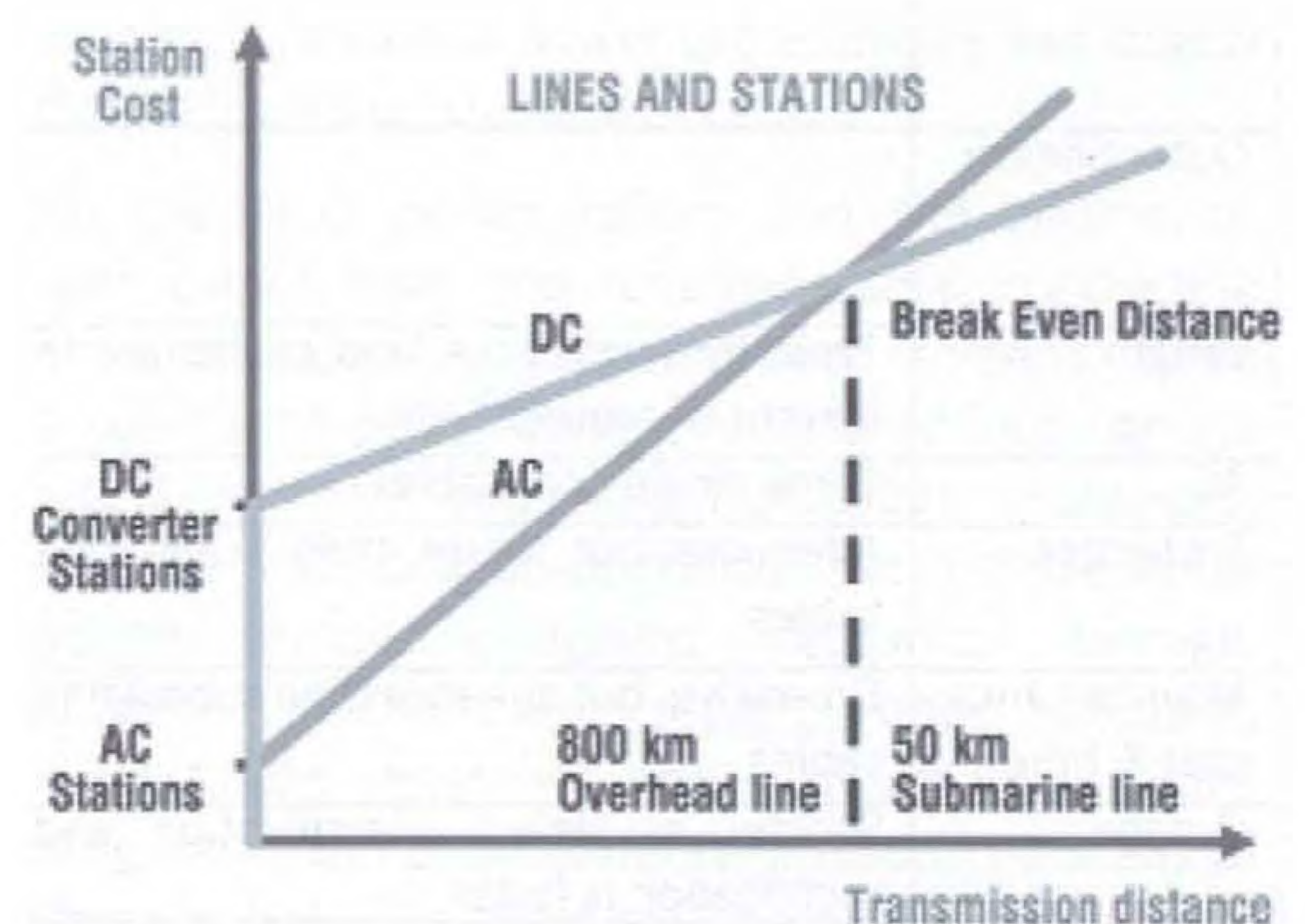
Figure-5: Comparative HVAC and HVDC costs (source: Electrical engineering portal [5])
